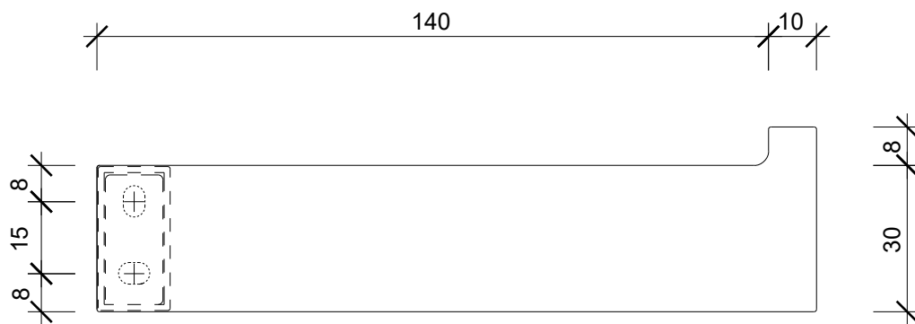
Frontansicht front view
